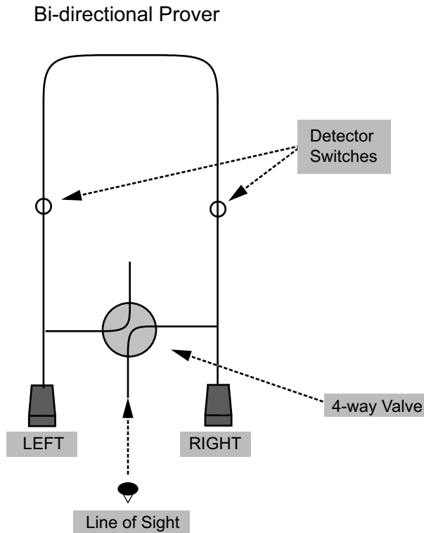
Figure 1—Bi-directional Prover Orientation of “Left” and “Right”
