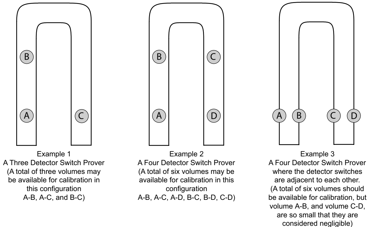
Figure 2—Examples of Multi-volume Prover Detector Switch Configurations
